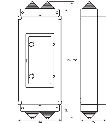
DFL8 Enclosure
